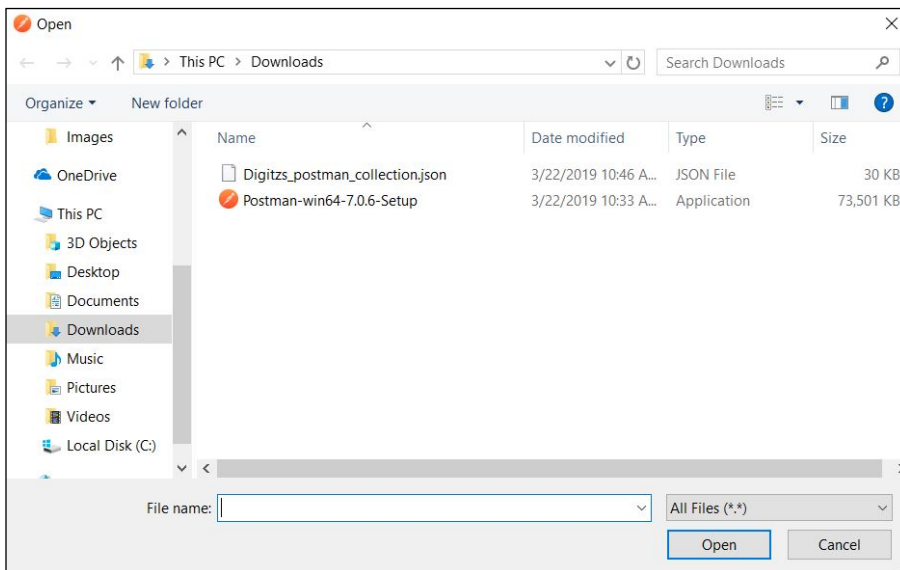
Figure 2 – Open Dialog
