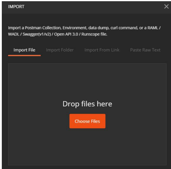
Figure 1 – Import Dialog
